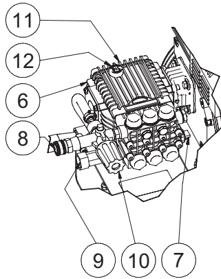
UNLOADER W/BYPASS
